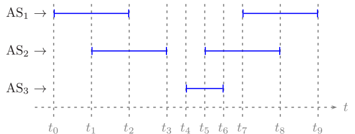
Fig. 1: Example of announcements for a prefix p
