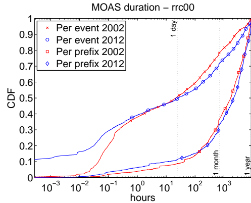
Fig. 2: MOAS events duration
