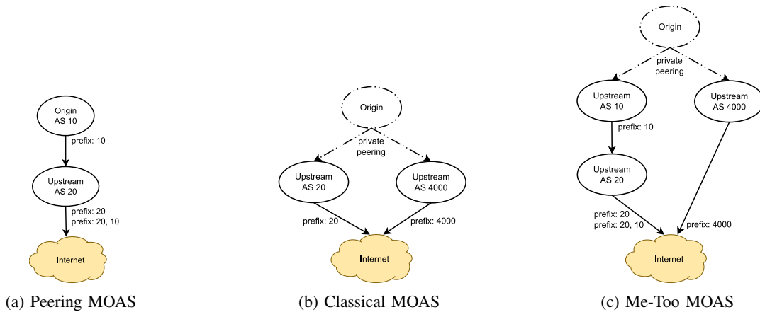
Fig. 4: Graphs of MOAS patterns
