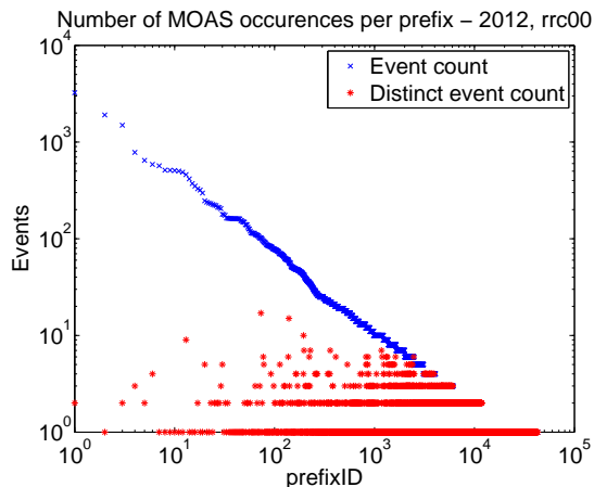
Fig. 3: Number of MOAS events per prefix
