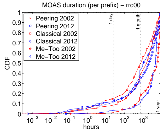
Fig. 5: MOAS patterns duration (per prefix)
